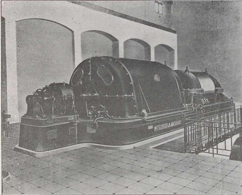
8,000 K. W. Turbo Generator for the Kinugawa Denki Kaisha, Ltd., manufactured at the Nagasaki Works.
