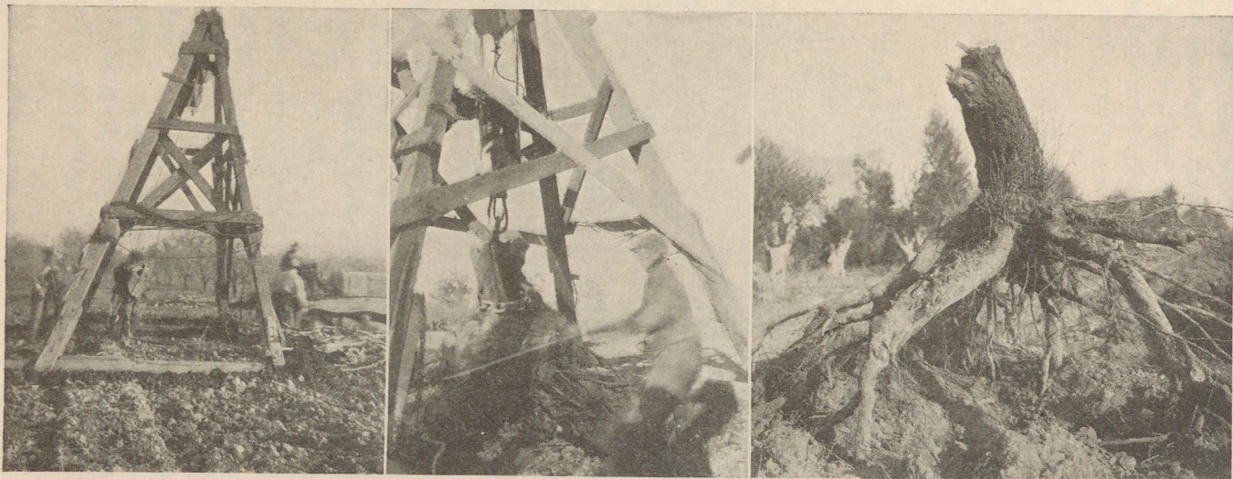
Fig. 8.—Derrick stump puller in operation. The illustrations show the beginning of the pull, the stump part way out of the ground, and the stump entirely out.
